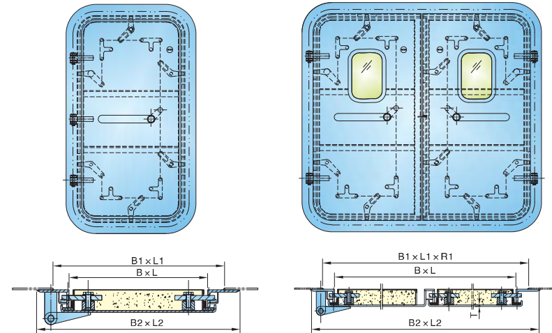
A60快开闭风雨密钢质门(单) A60快开闭风雨密钢质门(双) A60 QUICK OPEN & CLOSE WEATHERTIGHT STEEL DOOR ( SINGLE ) A60 QUICK OPEN & CLOSE WEATHERTIGHT STEEL DOOR ( DOUBLE )
