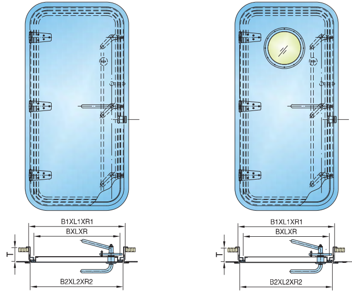
A型 - 快开闭风雨密铝质门 B型 - 快开闭风雨密铝质门 TYPE A QUICK OPEN & CLOSE WEATHERTIGHT ALUMINIUM DOOR TYPE B QUICK OPEN & CLOSE WEATHERTIGHT ALUMINIUM DOOR
